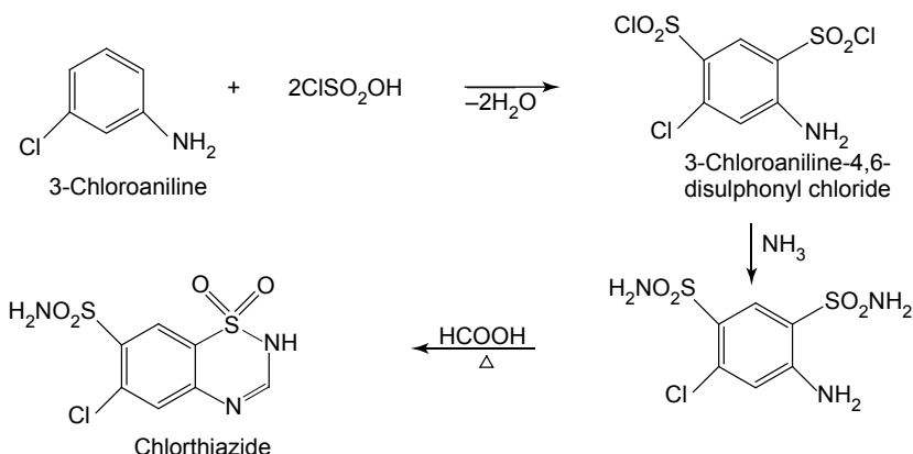
6-Chloro-1,2,4-benzothiazine-7-sulphonamide-1,1-dioxide
