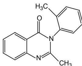
2-Methyl-3-o-tolylquinazolin-4(3H)-one
