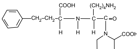
1-[N-2- [(S)-1-Carboxy-3-phenyl propyl]-L-lysyl]-L-proline dihydrate
