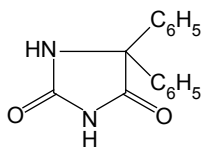
Phenytoin
