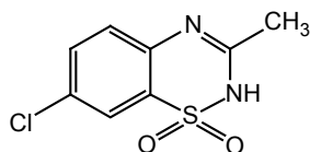
7-Chloro-3-methyl-2H-1,2,4-benzothiadiazine-1,1-dioxide
