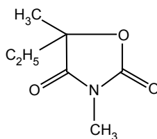
5-Ethyl-3,5-dimethyl oxazolidine-2,4-dione
