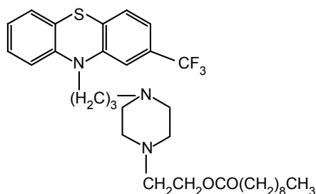
Fluphenazine deconoate
