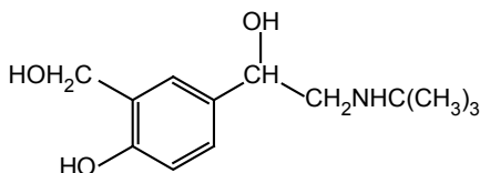
4-Hydroxy-3-hydroxy methyl- \alpha -[(tert butylamino)methyl]benzyl alcohol
