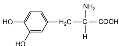
2-Amino-3-(3,4-dihydroxyphenyl) propanoic acid
