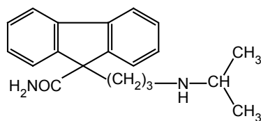
ropafenone
