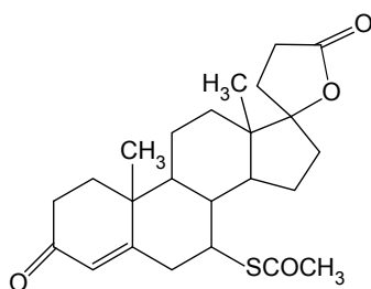
Spironolactone
