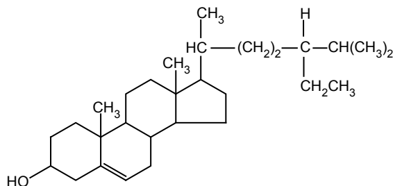
3- \beta -stigmasterol-5-en-3-ol
