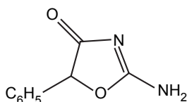
2-Amino-5-phenyloxazol-4(5 H )-one
