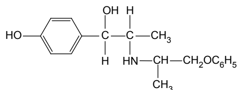
4-(1-Hydroxy-2-(1-phenoxypropyl-amino)propyl) phenol
