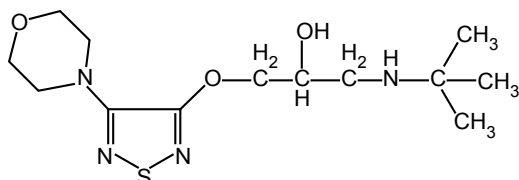
Timolol
