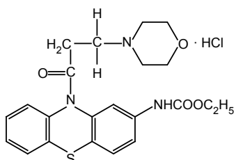
Ethyl-10-(3-morpholinopropanoyl)-phenothiazin-2-yl-carbamate hydrochloride
