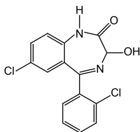
7-Chloro-5-(2-chlorophenyl)-3-hydroxy-1,4-benzodiazepin-2-one
