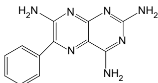
2,4,7-Triamino-6-phenylpteridine
