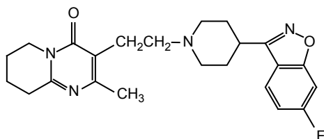
3-[2-[4-(6-Fluoro-1,2-benzisoxazol-3-yl)-1-piperidinyl]ethyl]6,7,8,9-tetrahydro-2-methyl-4H-pyrido(1,2-a)pyrimidin-4-one
