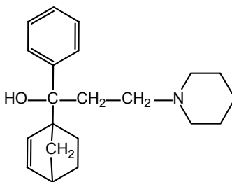
1-(Bicyclo hept-2-en-1-yl)-1-phenyl-3-(piperidin-1-yl)propan-1-ol
