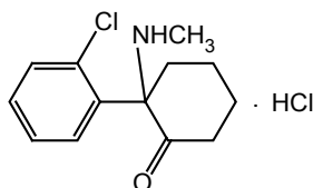
2-(2-Chloro phenyl)-2-(methlamino) cyclohexanone
