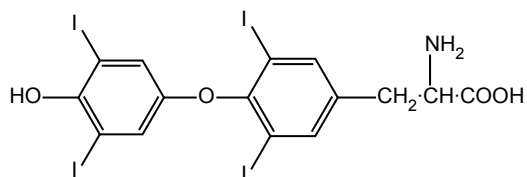
o -(4-Hydroxy-3,5-diiodophenyl)-3,5-diiodo-D-tyrosine
