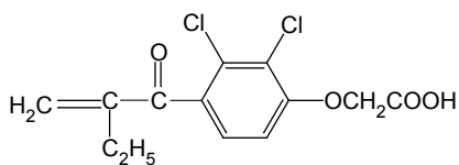
Ethacrynic acid
